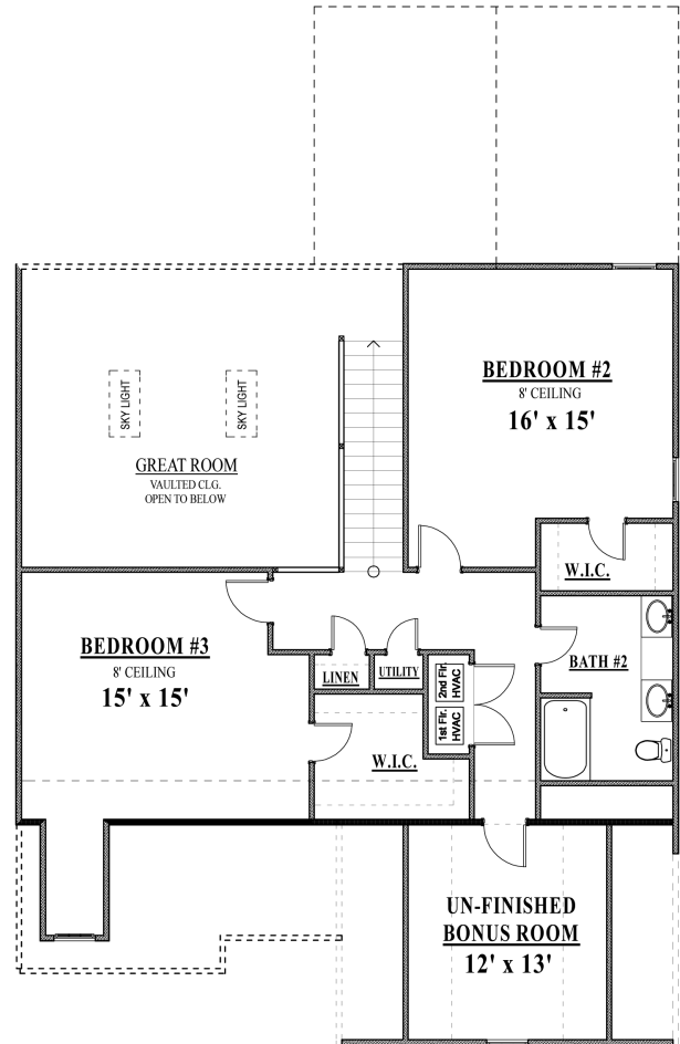
Second Floor 969 Sq. Ft.
