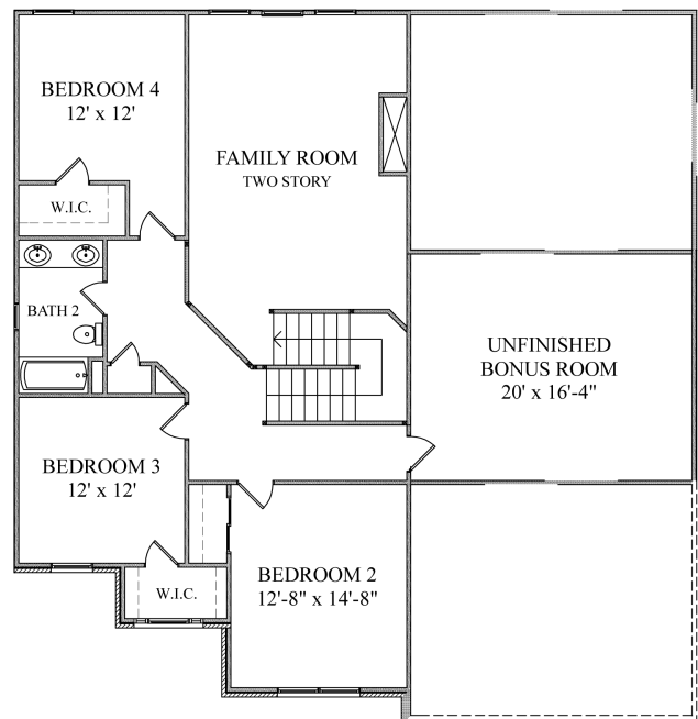
Second Floor 816 Sq. Ft.
