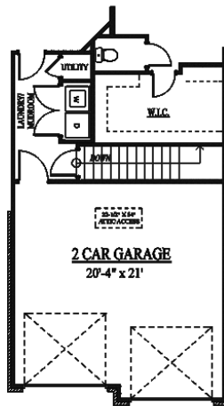
Basement Layout
