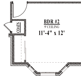
ALTERNET LAYOUT WITH BAY WINDOW
