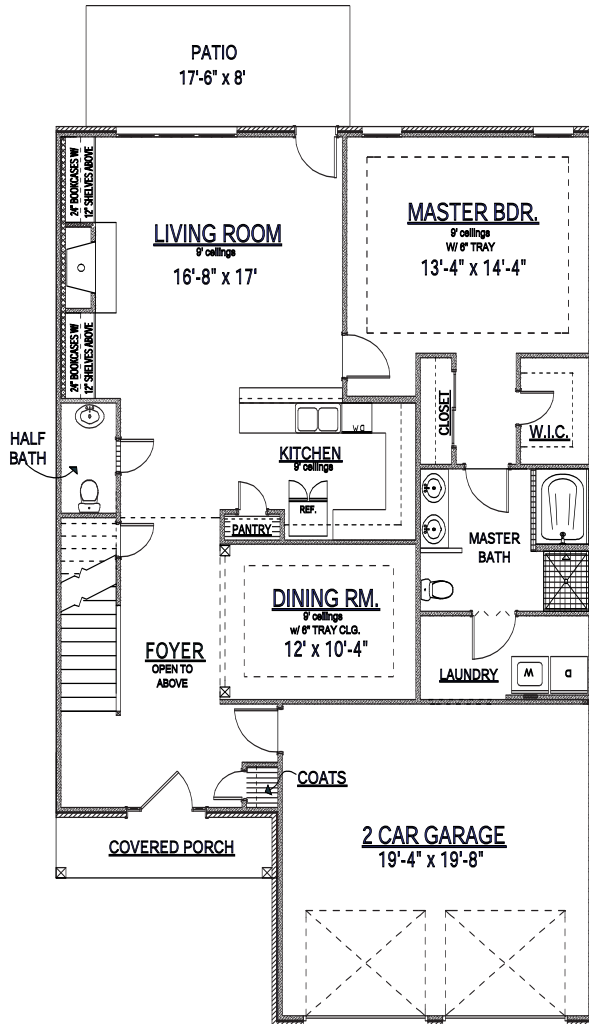
First Floor 1,478 Sq. Ft.
