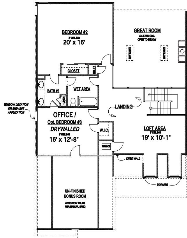
Second Floor 1,160 Sq. Ft.
