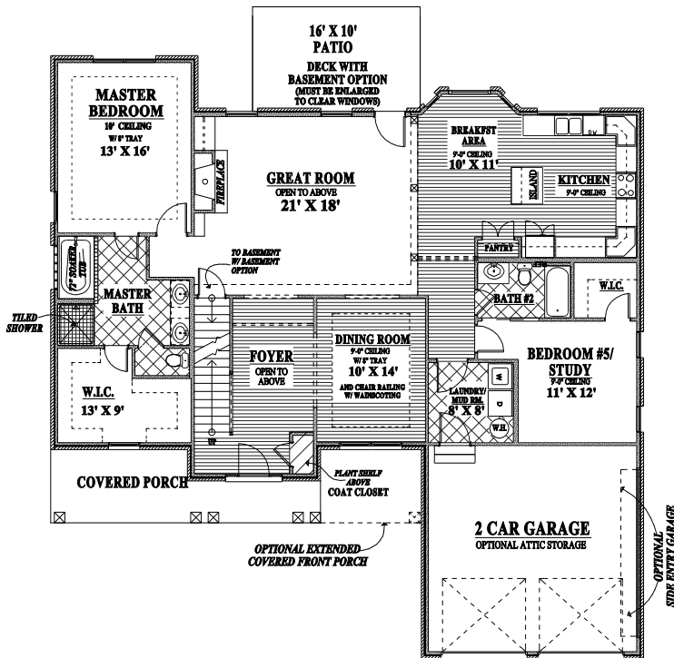
First Floor 1924 Square Feet
