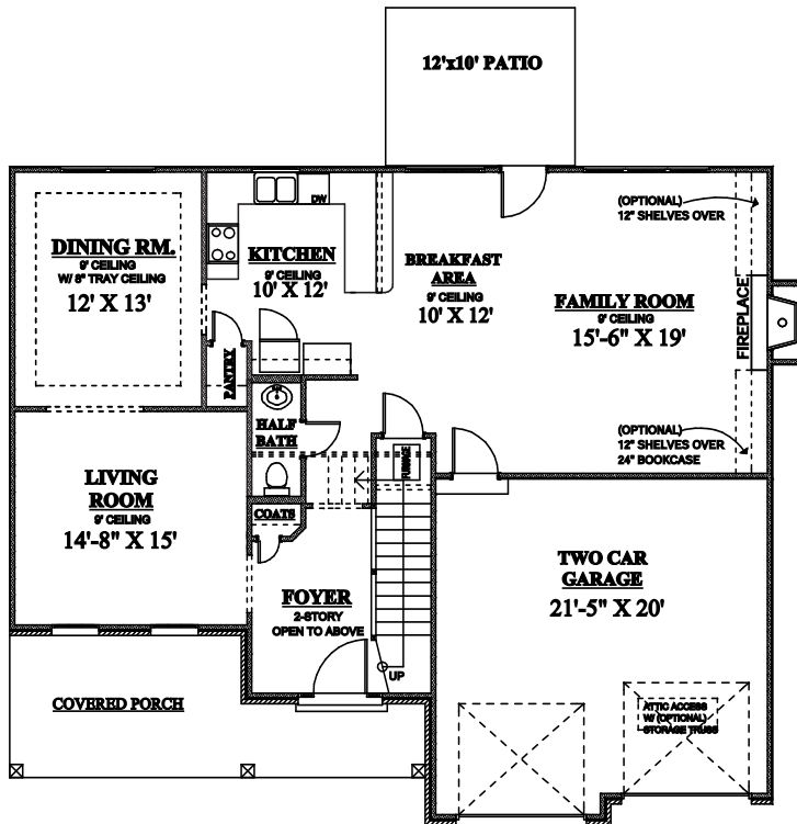
First Floor 1257 Sq. Ft.
