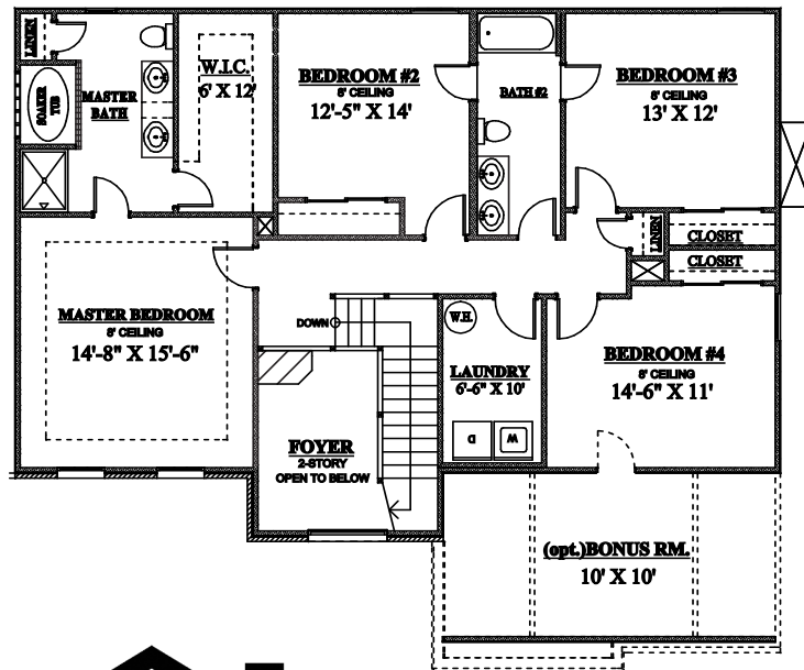
Second Floor 1294 Sq. Ft.
